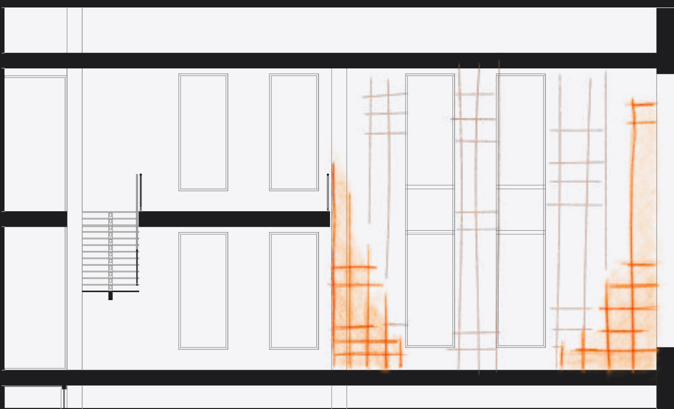
1:100 Section
